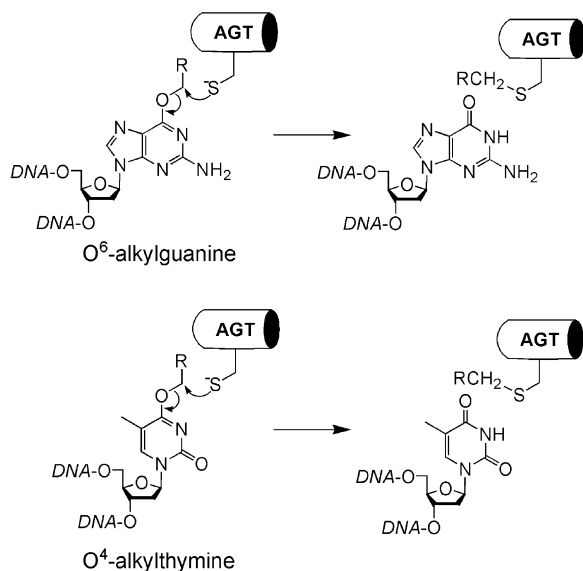
Figure 1. DNA Repair Functions Performed by O^6 -Alkylguanine-DNA Alkyltransferases
